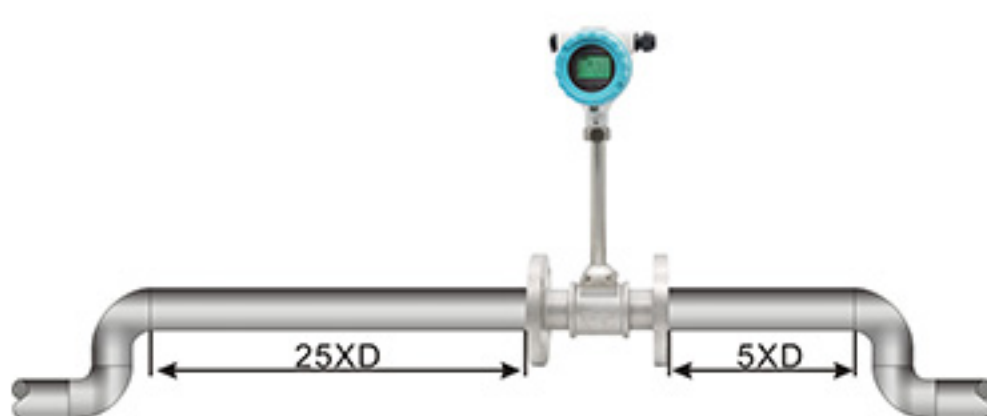
Two Square Bends At Same Plane
